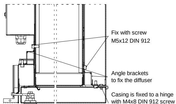
Cut G-G
