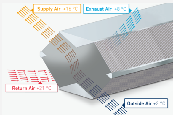
Heat exchanger
