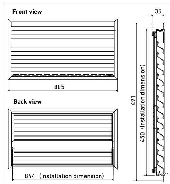
Weather protection grille
