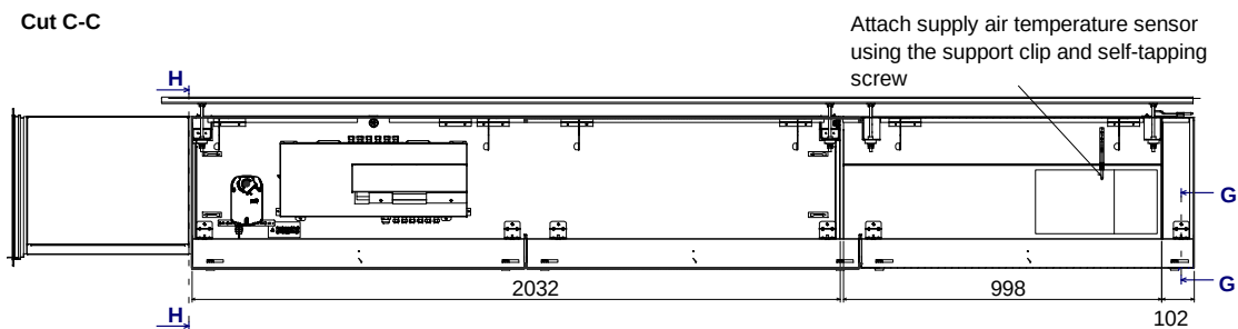
Cut C-C
