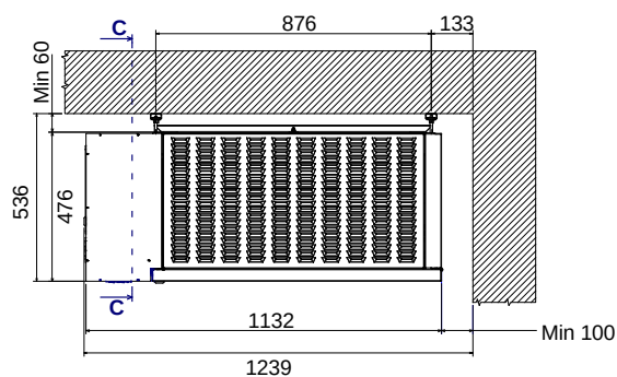
View exhaust air side
