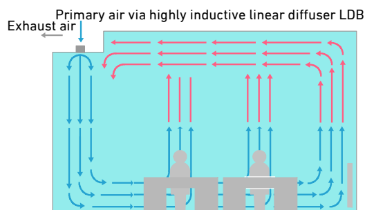
Mixed-displacement flow (type FVS-DI)
