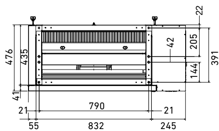
Cut H-H
